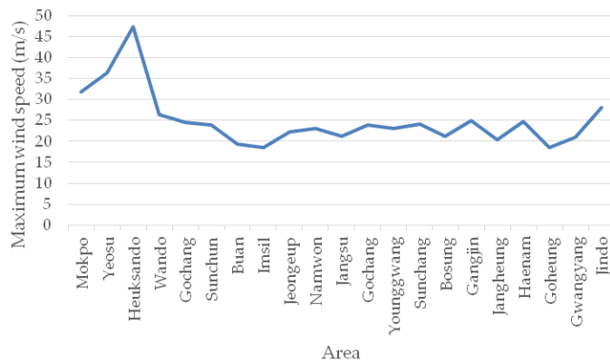
Figure 4: Maximum instantaneous wind speed (m s) in the Seomjin and Yeongsan River areas (2020-2023).
