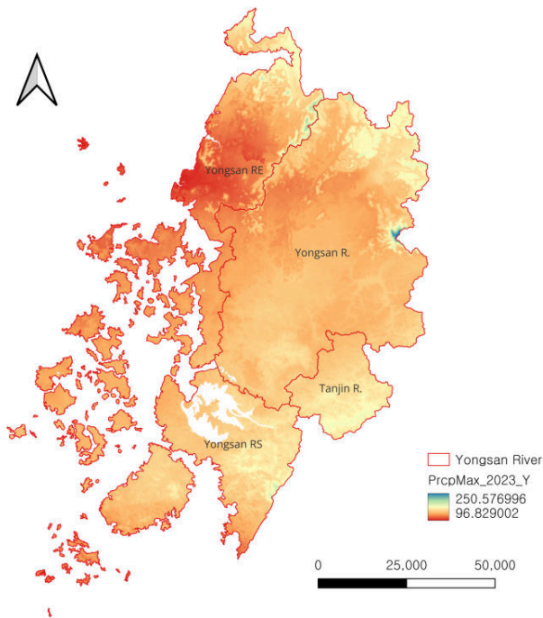
Figure 11: Gridded maximum precipitation over the Yeongsan River basin (2020-2023).
