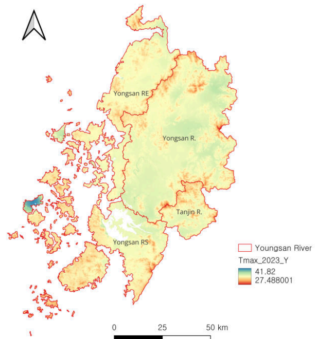
Figure 9: Gridded maximum temperature over the Yeongsan River basin (2020-2023).
