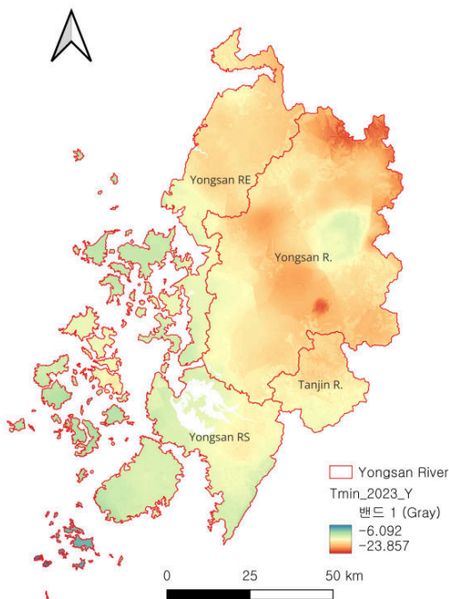
Figure 7: Gridded minimum temperature over the Yeongsan River basin (2020-2023).
