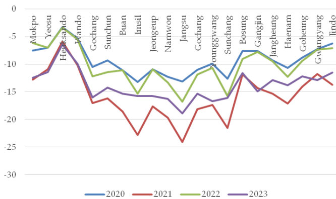
Figure 1: Annual distribution of daily minimum temperature at observation points within the Seomjin and Yeongsan River basins (2020-2023).
