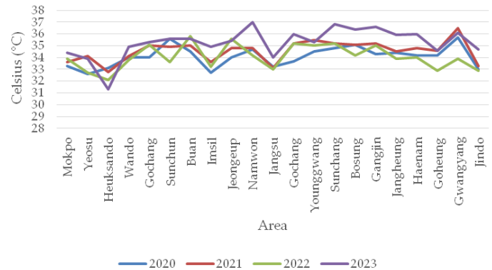
Figure 2: Annual distribution of daily maximum temperature at observation points within the Seomjin and Yeongsan River basins (2020-2023).
