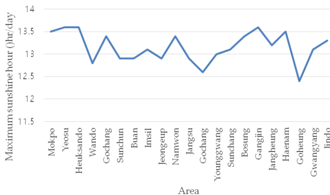
Figure 5: Observed daily maximum sunshine duration at monitoring stations in the Seomjin and Yeongsan River basins (2020-2023).
