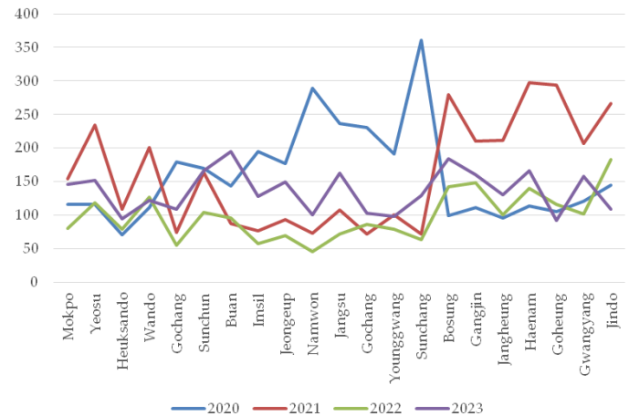
Figure 3: Annual distribution of maximum daily precipitation at observation points within the Seomjin and Yeongsan River basins (2020-2023).
