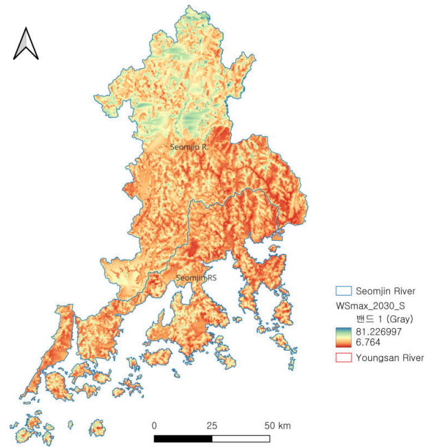
Figure 12: Gridded maximum instantaneous wind speed (m s) over the Seomjin River basin (2020-2023).
