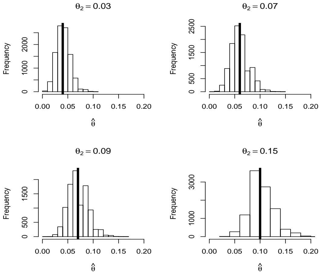
Figure 3: Histograms of misclassification estimates, \hat{\theta} . \theta_1 = 0.05 and p = 0.5 in each histogram. The thick vertical line represents the average misclassification rate.
