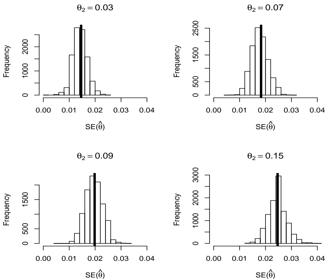
Figure 4: Histograms of the standard error of misclassification estimates, SE(\hat{\theta}) . \theta_1 = 0.05 and p = 0.5 in each histogram. The thick vertical line represents the sample standard deviation of the simulated misclassification probability estimates.
