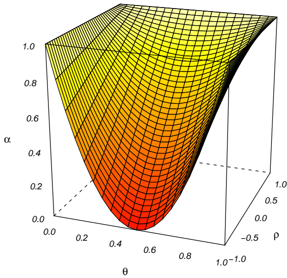
Figure 2: Interpreter agreement ( \alpha ) as a function of misclassification probability ( \theta ) and the correctness correlation ( \rho ).
